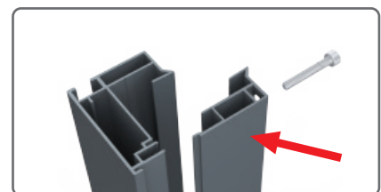
Separate tracks and concealed screws. much easier assemble and disassemble
